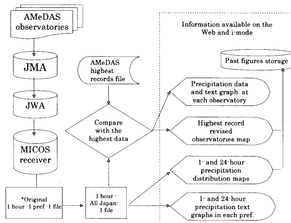
Fig. 1 Outline of the Real-time Heavy Rainfall Display System.
